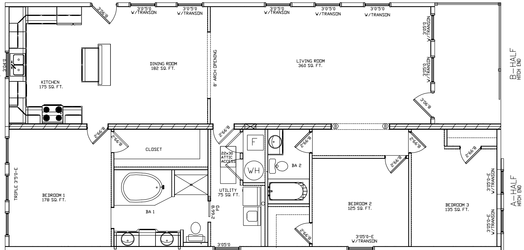
MODEL 1054-M0 30X60 3 BR - 2 BATH APPROX. 1,764 SF
